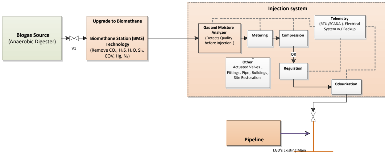
Figure 1: RNG Production Process and Enbridge Service Offerings
